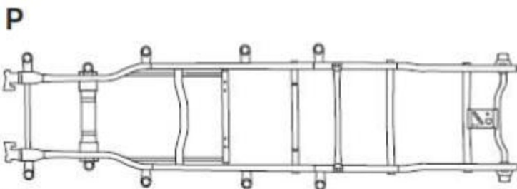
UNDERBODY VIEW
